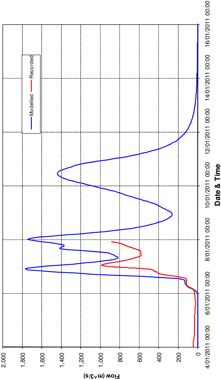
Brisbane River at Gregors Creek 22:00 on 7 January 2011
