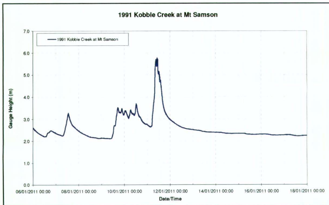
Figure 6.7.4 – Gauge height, Kobble Creek at Mt Samson Road
