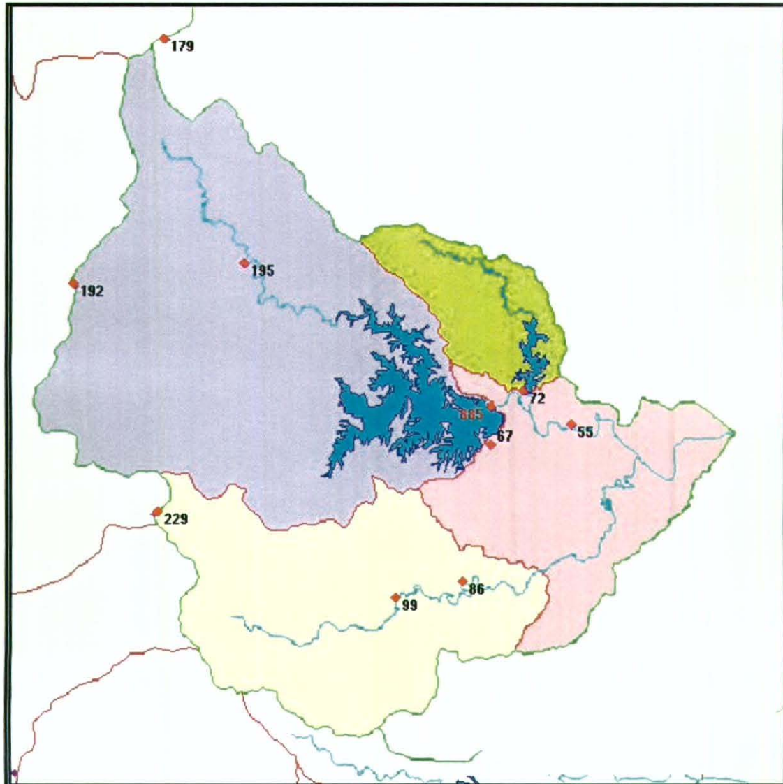
Figure 6.2.8 – Rainfall in the 24 hours to 09:00 on Wednesday 12 January 2011
