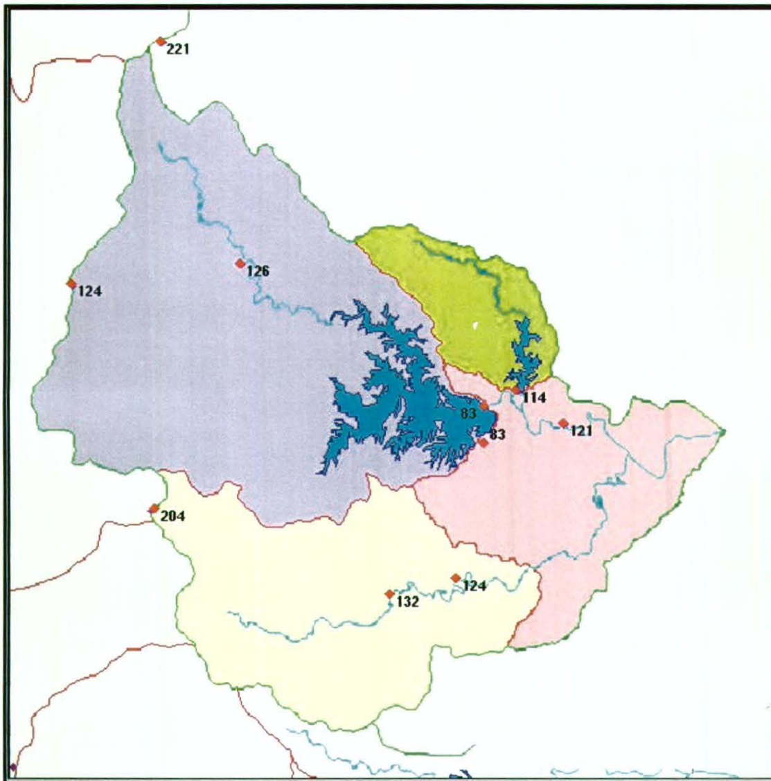
Figure 6.2.6 - Rainfall in the 24 hours to 09:00 on Monday 10 January 2011
