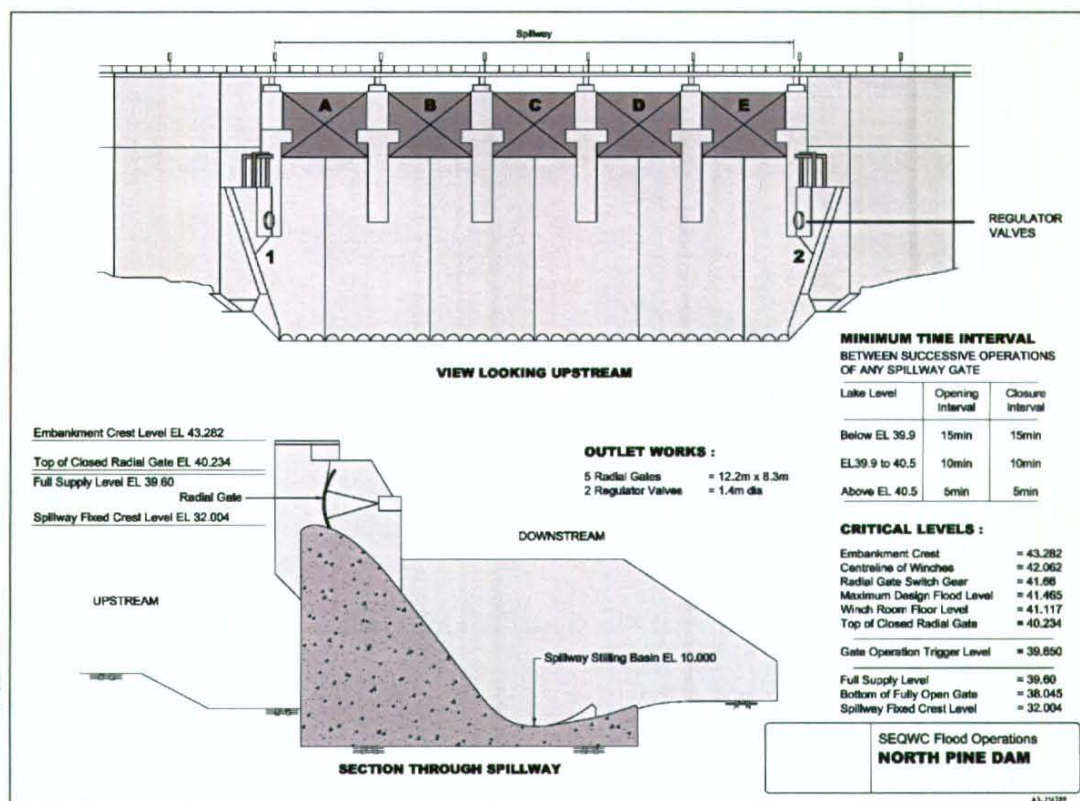
Figure 1.4.1 – North Pine Dam infrastructure – arrangement of the radial gates
