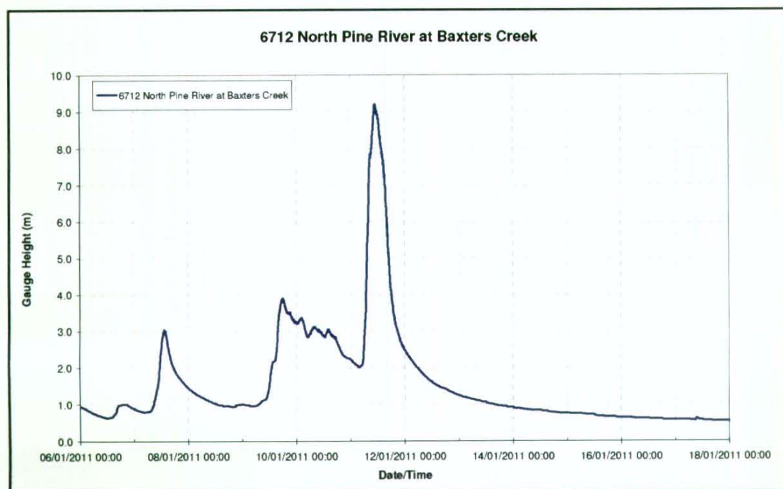
Figure 6.7.2 – Gauge height, North Pine River at Baxters Creek
