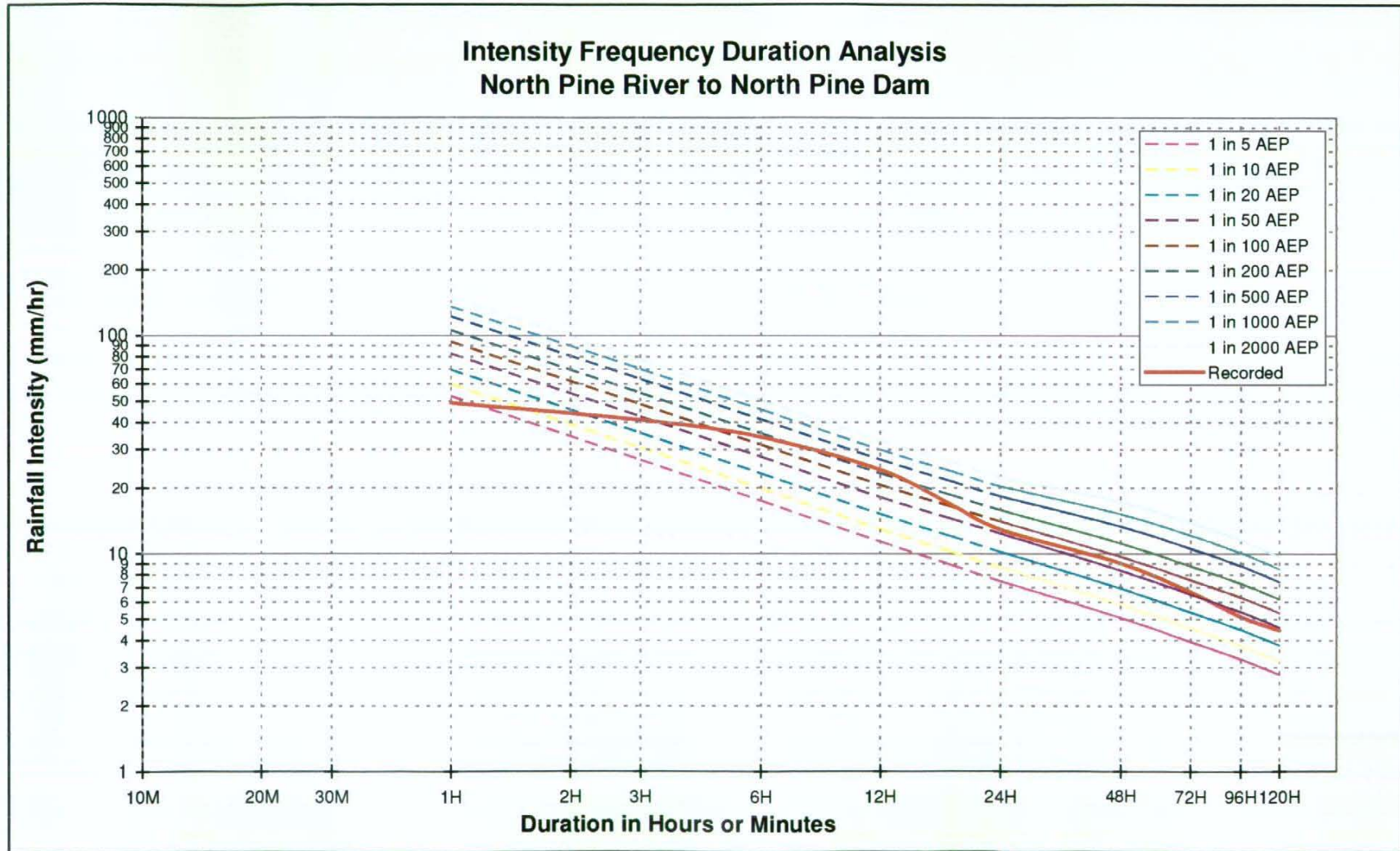
Figure 9.4.2 – Rainfall intensity, North Pine Dam
