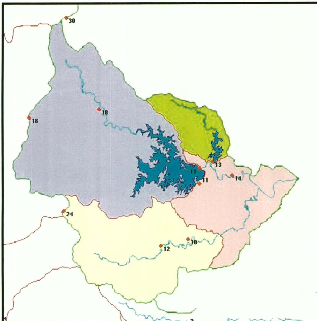
Figure 6.2.5 - Rainfall in the 24 hours to 09:00 on Sunday 9 January 2011
