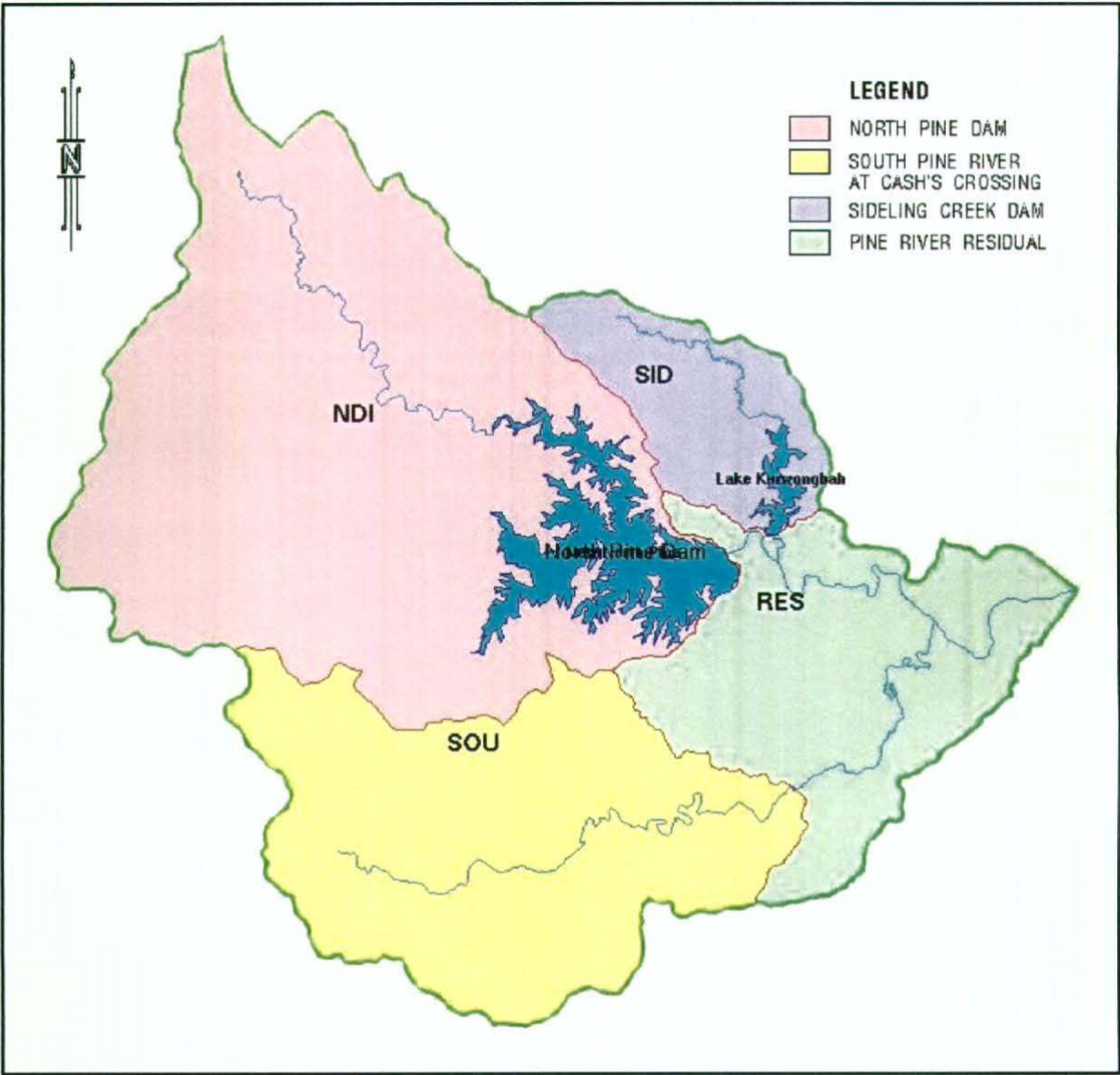
Figure 7.2.1 – RTFM Regions
