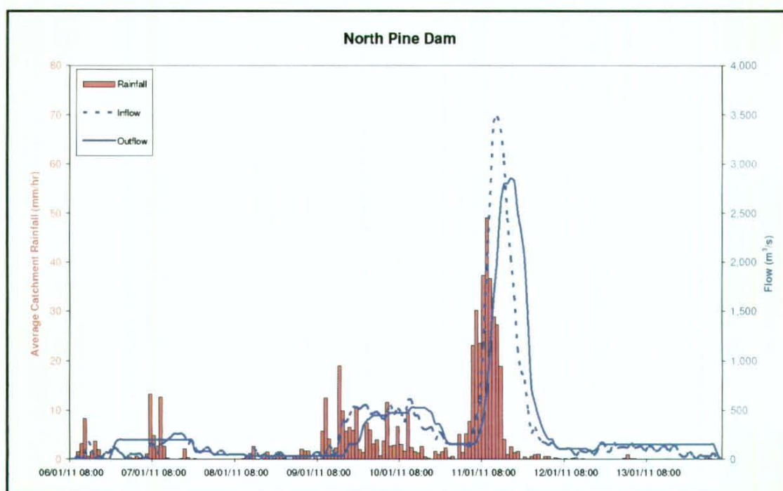
Figure 2.1.1 – North Pine Dam – January 2011 Flood Event – Dam inflow and outflow
