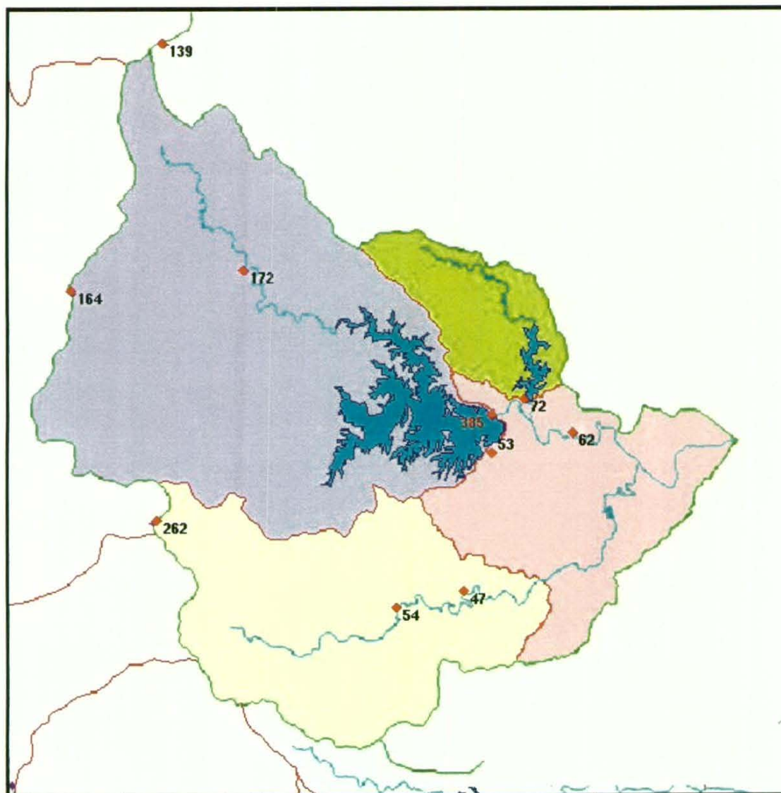
Figure 6.2.7 - Rainfall in the 24 hours to 09:00 on Tuesday 11 January 2011
