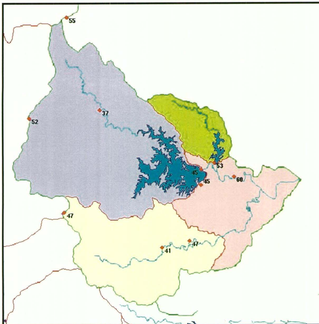
Figure 6.2.3 - Rainfall in the 24 hours to 09:00 on Friday 7 January 2011
