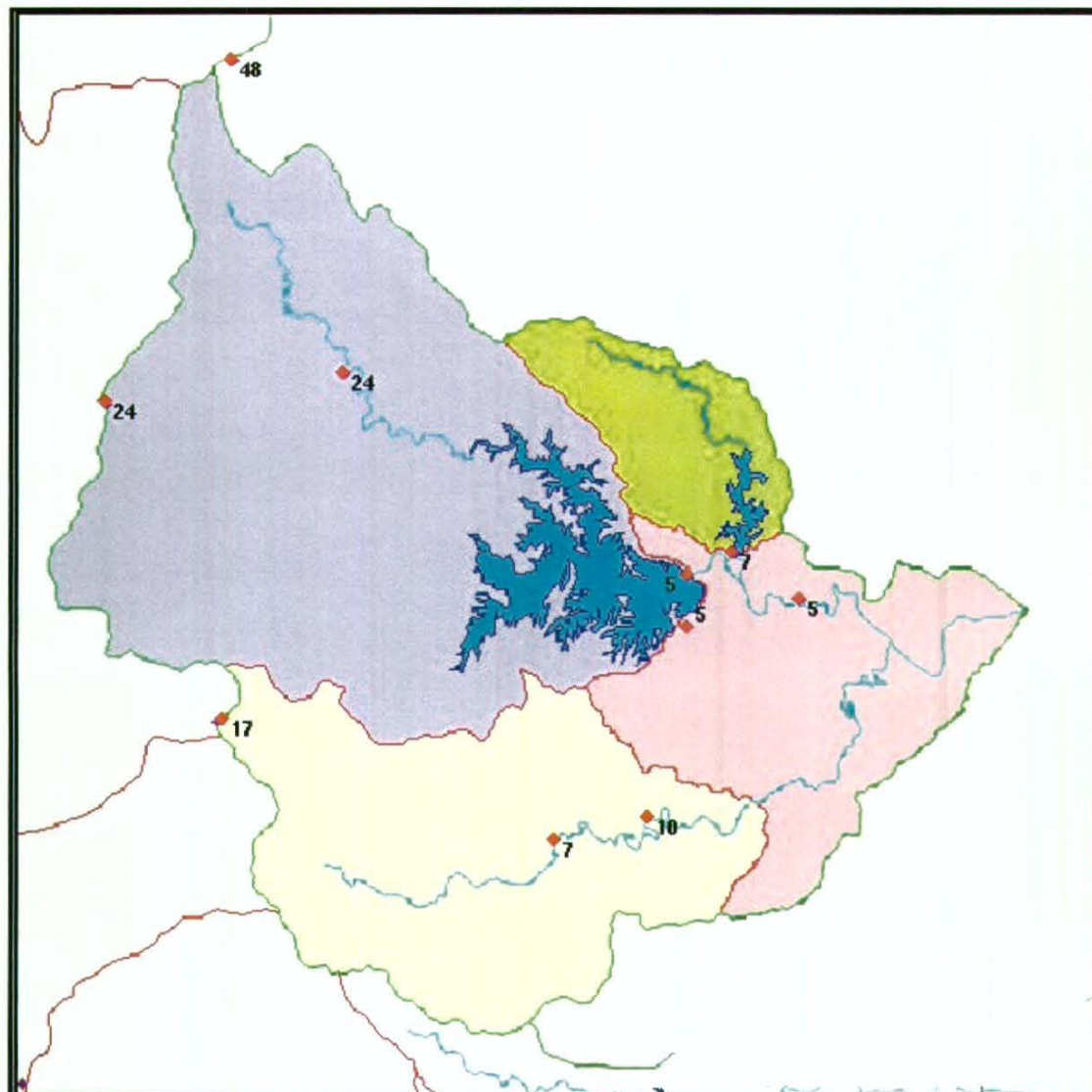
Figure 6.2.4 - Rainfall in the 24 hours to 09:00 on Saturday 8 January 2011
