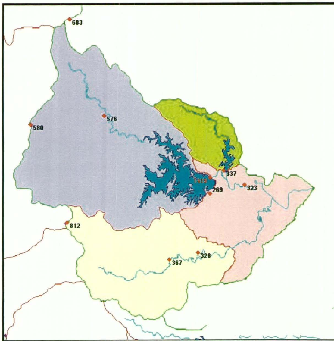
Figure 6.2.9 - Rainfall in the seven days to 09:00 on Wednesday 12 January 2011
