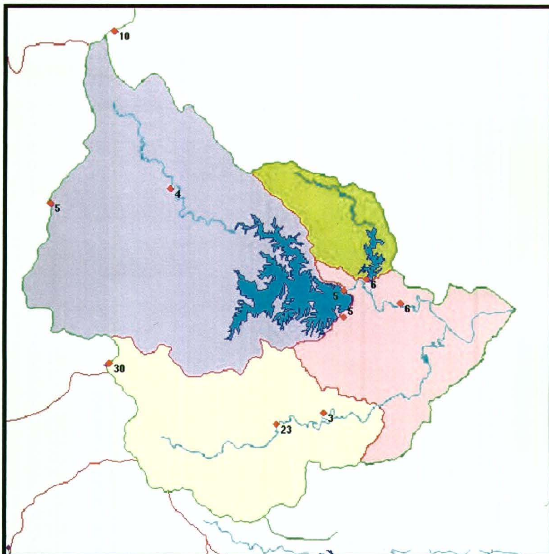
Figure 6.2.2 - Rainfall in the 24 hours to 09:00 on Thursday 6 January 2011
