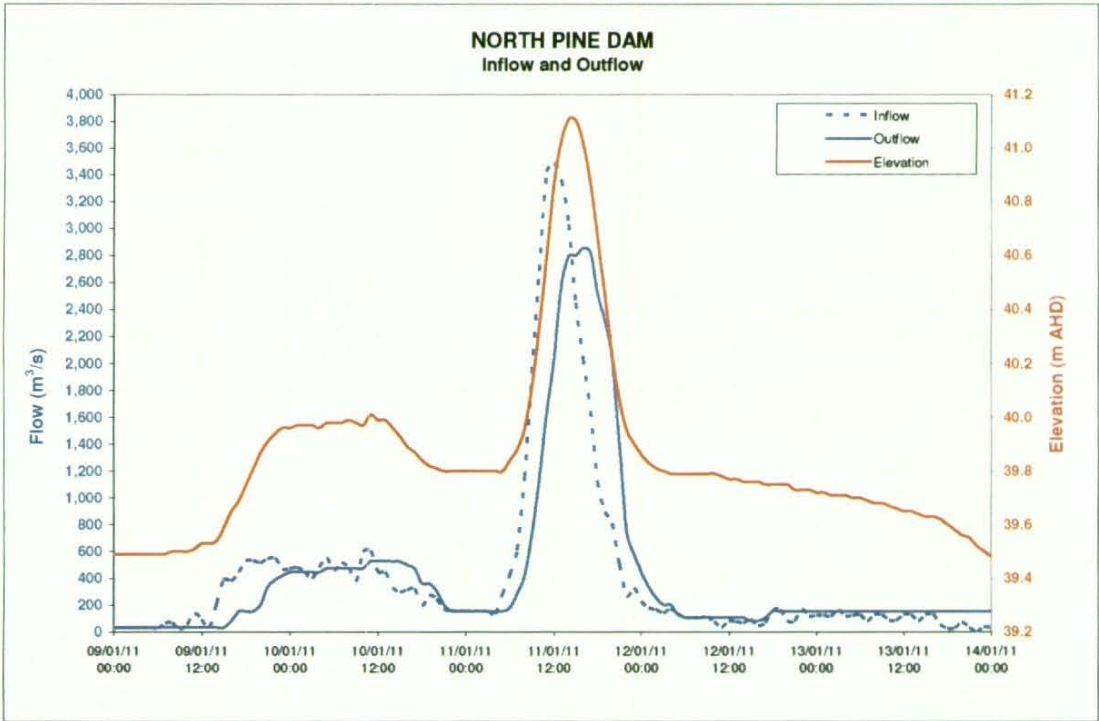
Figure 6.8.2 – North Pine Dam inflow and outflow
