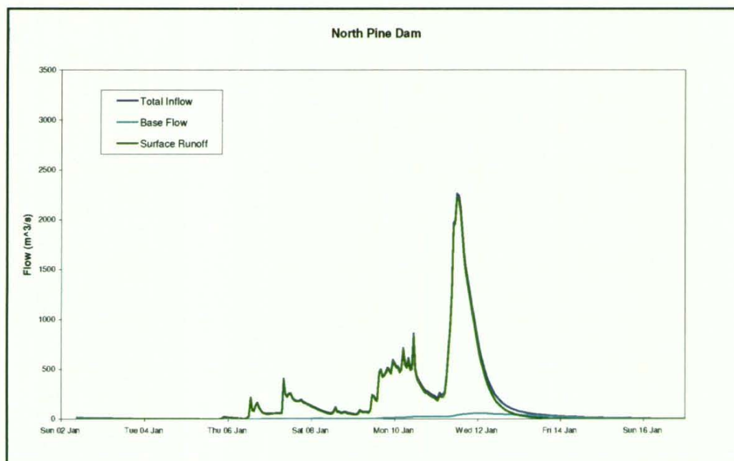
Figure 7.2.4 – Modelled inflow into North Pine Dam
