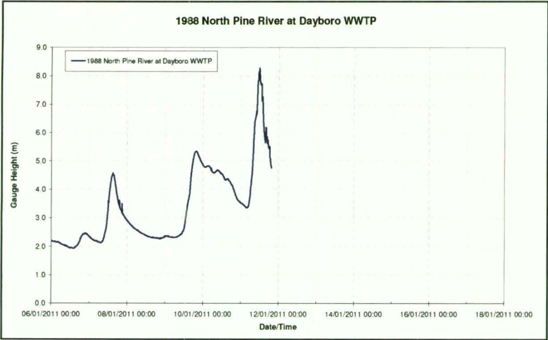
Figure 6.7.3 – Gauge height, North Pine River at Dayboro WTPP
